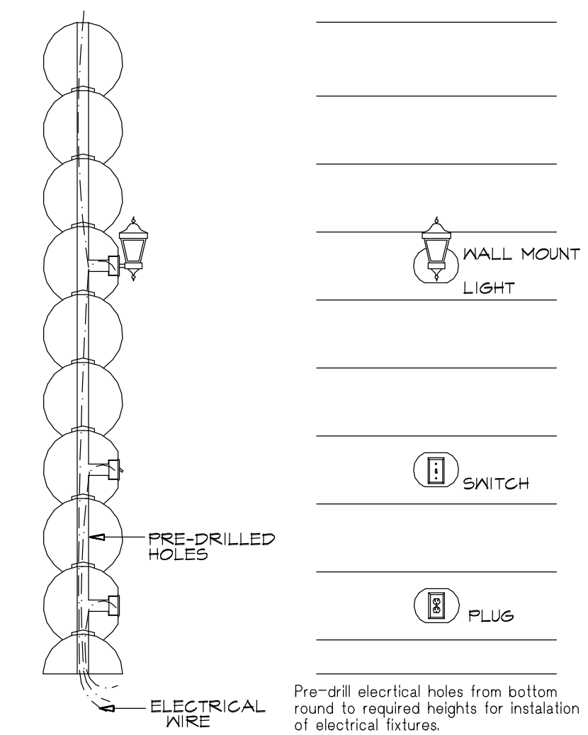
11 TYPICAL ELECTRICAL A.12 N.T.S.
